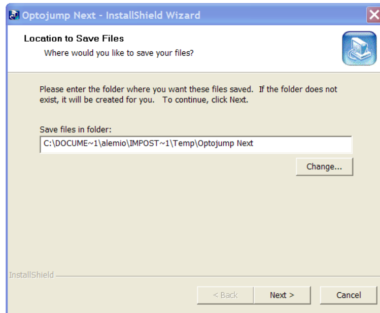
Abb. 2– Installationsassistent
