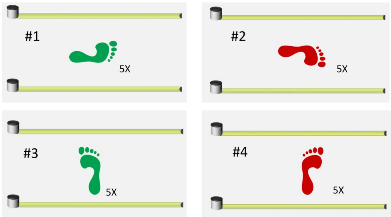
Abb. 111 - Drift-Protokoll-Sequenz
