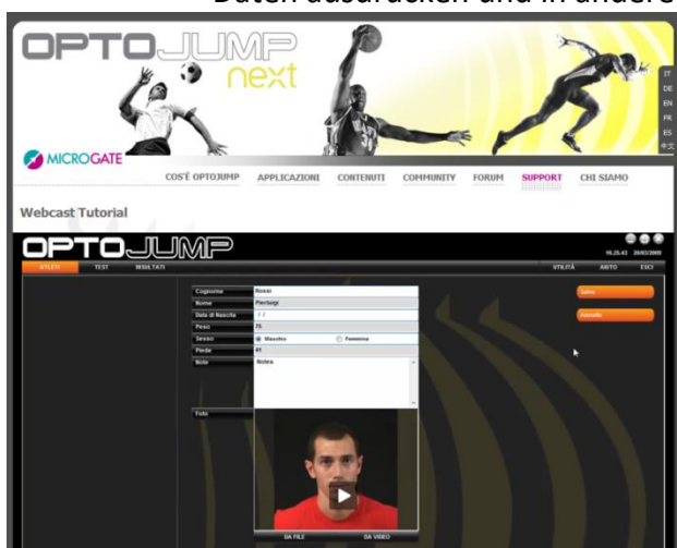
Abb. 1 – Webcast-Tutorial
