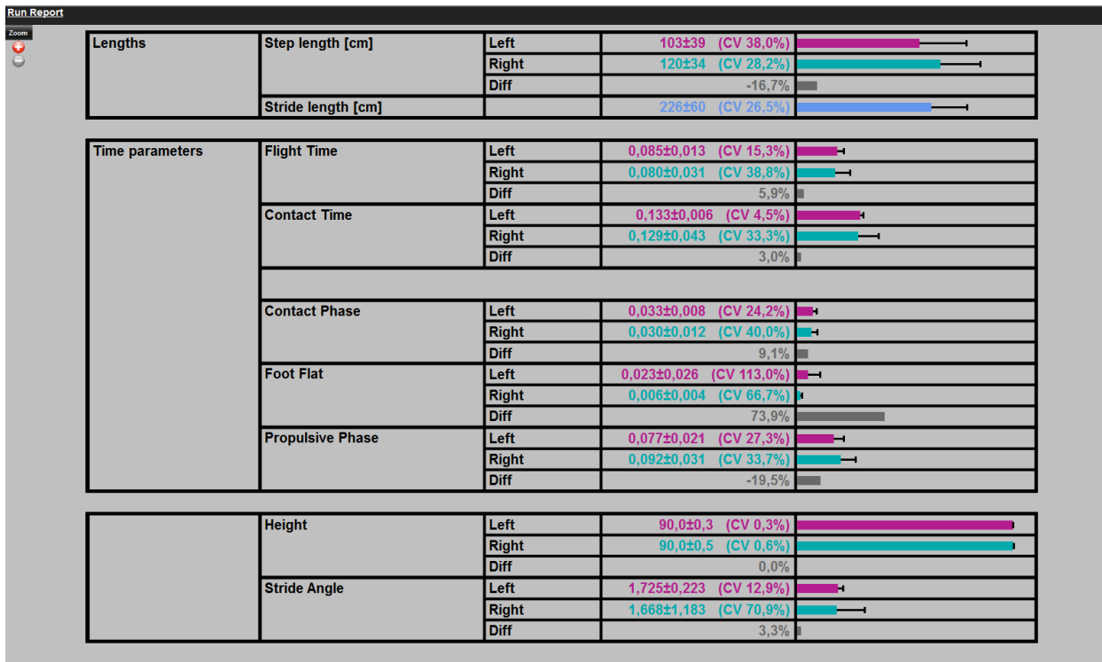
Abb. 61 - Run Report
